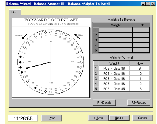
One easy to read display shows the size and location of balance weights to install.
