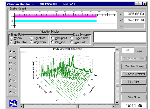
Waterfall spectra identify changes during speed changes.
