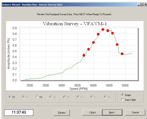
Pre-defined balancing speeds highlighted on a vibration survey graph.
