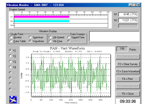
The oscilloscope display can be used to detect faulty sensors and other problems.
