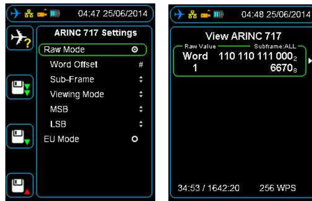
Figure 17.0 ARINC 717 settings
