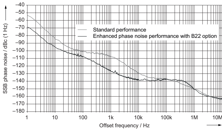
Measured SSB phase noise, f = 1 \text{ GHz} , comparison of standard performance and performance with R&S ® SMA-B22 option.
