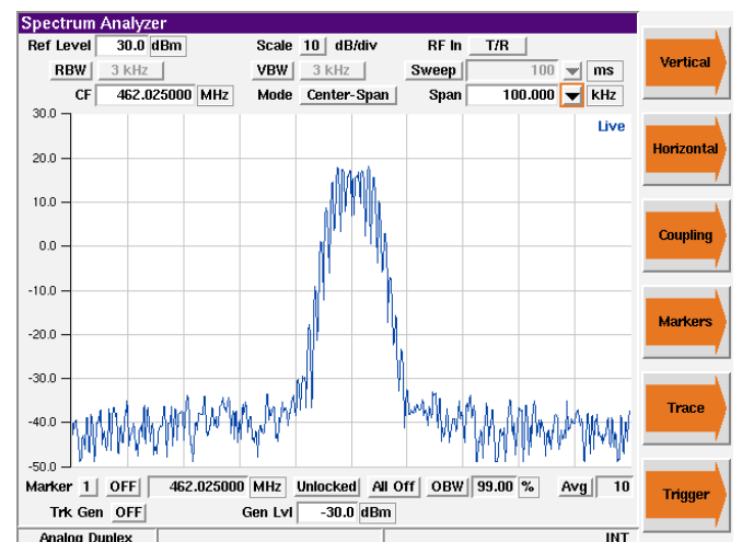
Figure 5. Spectrum Analyzer
