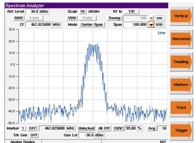
Figure 5. Spectrum Analyzer
